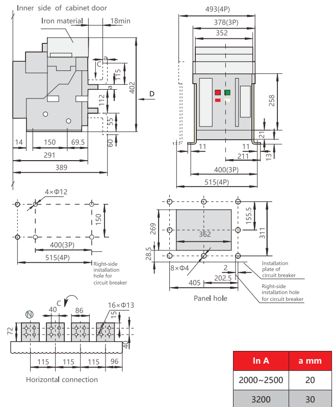
2 nd frame(2000~3200A) Fixed - Horizontal Rear Terminal
