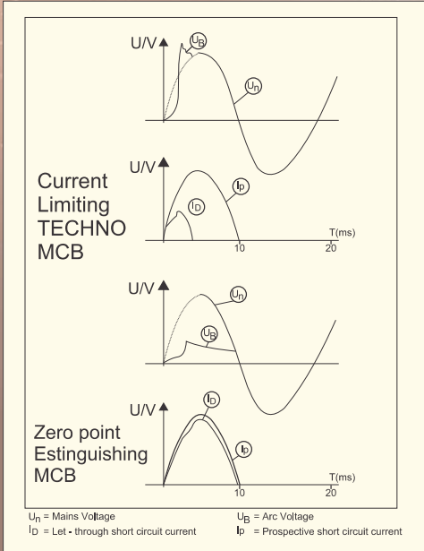
Techno MCB Vs Zero Point Extinguishing MCB
