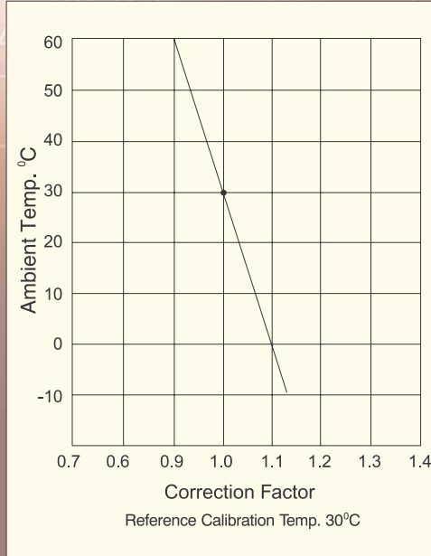
Temperature Compensation Graph
