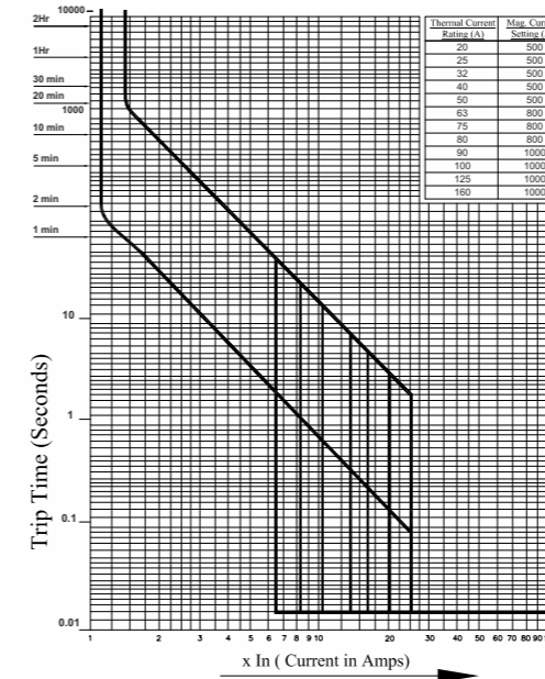
Time Current Characteristic Curve (TAB-2)
